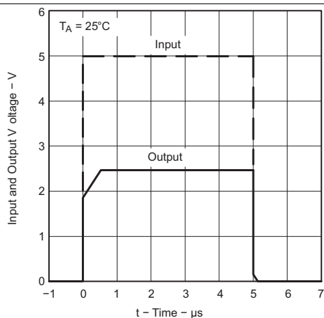
Figure 14. Pulse Response
